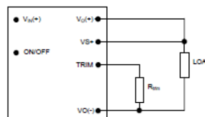
Figure 26. Circuit configuration for programming output voltage using an external resistor.
