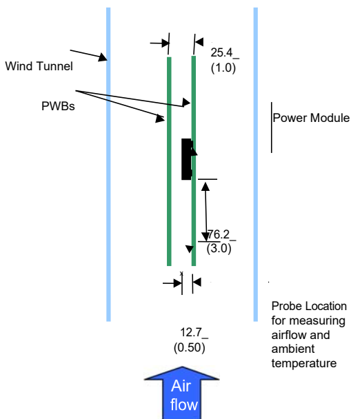
Figure 28. Thermal Test Setup.
