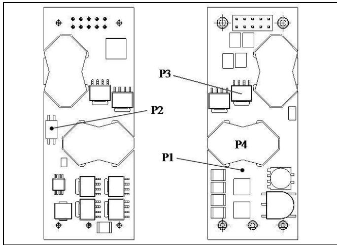
TOP View Open frame Bottom View Open frame and Baseplate (Best air flow direction is from negative to positive pins.)
