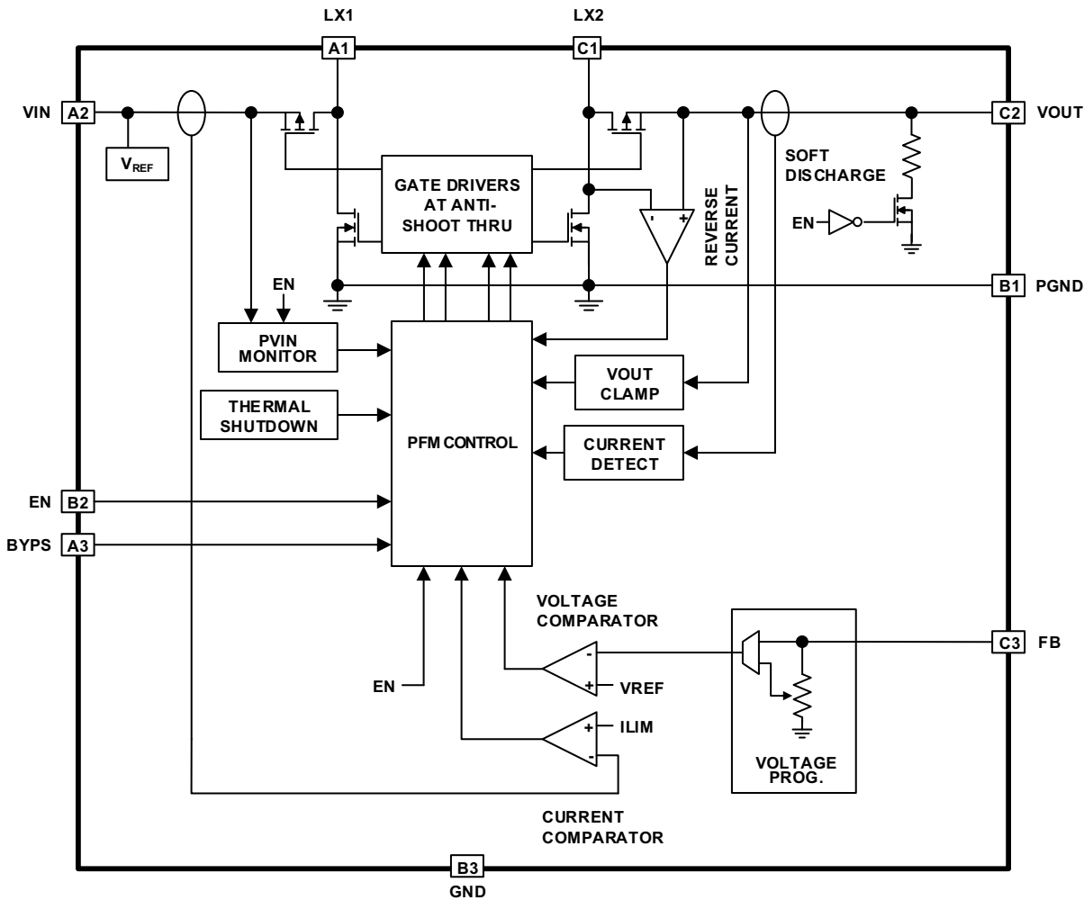
FIGURE 3. BLOCK DIAGRAM
