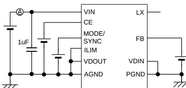
Circuit ②
