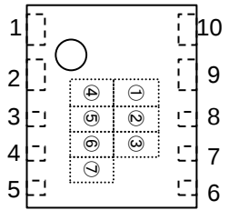
USP-10B (BOTTOM VIEW)
