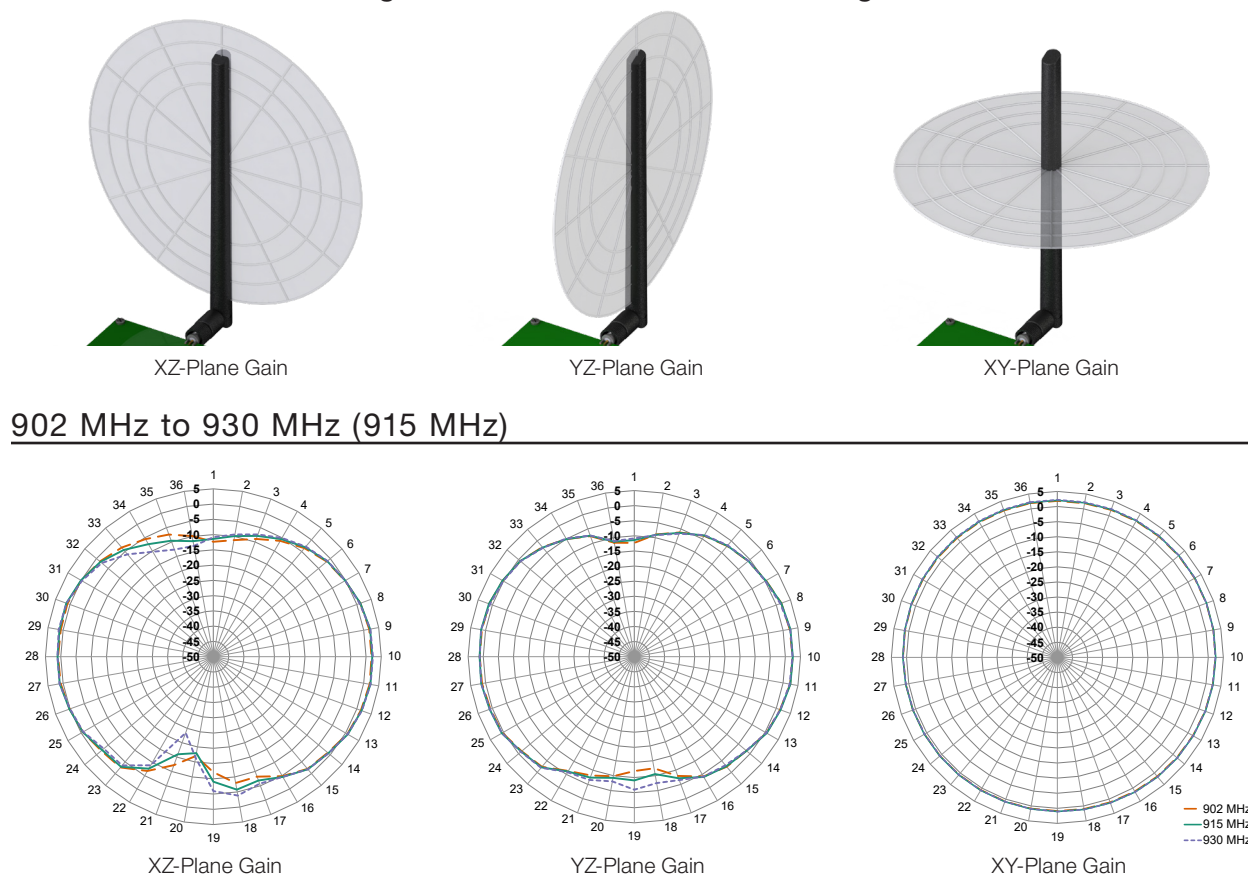
Figure 9. Radiation Patterns for ANT-915-IPW1-RPS, Edge Bent
