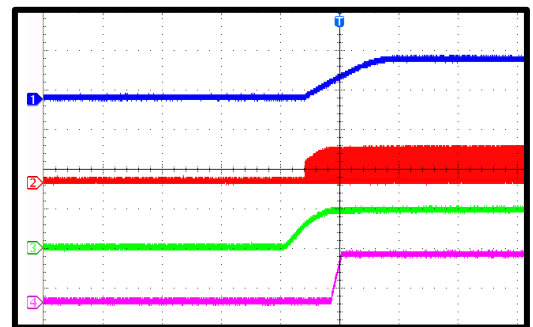
Start-Up through V_{IN}
