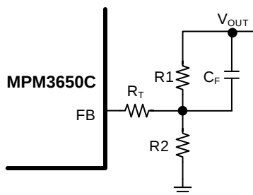
Figure 5: Feedback Network
