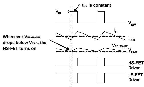
Figure 3: FCCM Operation
