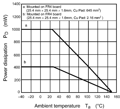
Fig. 8.13 P_D - T_a
