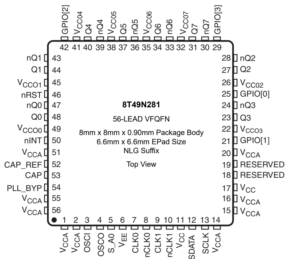
Figure 2. Pinout Drawing
