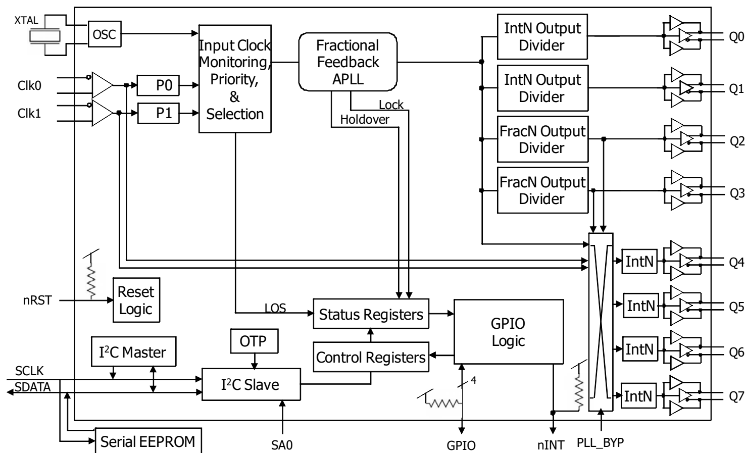
Figure 1. 8T49N281 Functional Block Diagram
