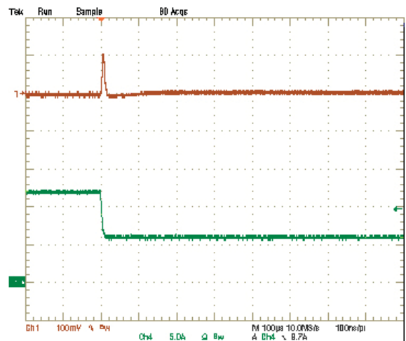
Step Load Transient Response (Vin=5.0V, Vout=3.3V, Cload=94μF, Iout=12A to 6A) Trace 1=Vout, 100 mV/div, Trace 4=Iout, 5A/div.
