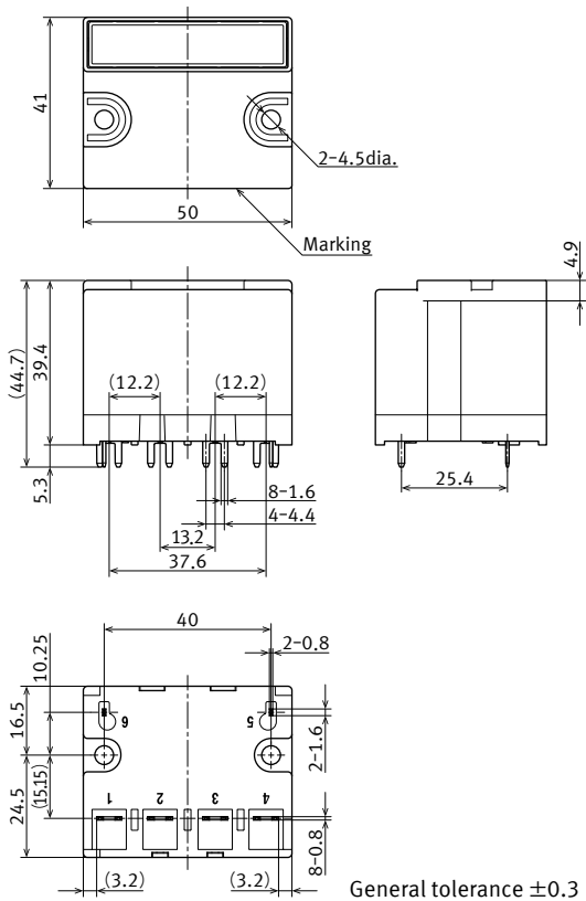
External dimensions
