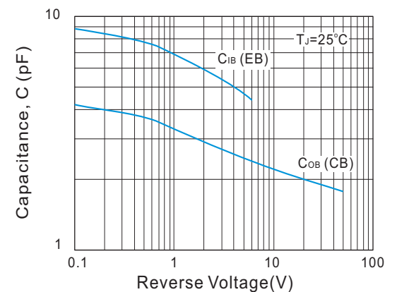
Fig. 6. Typical Capacitances vs. Reverse Voltage
