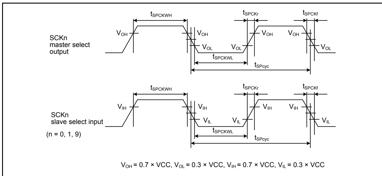
Figure 2.43 SCI simple SPI mode clock timing
