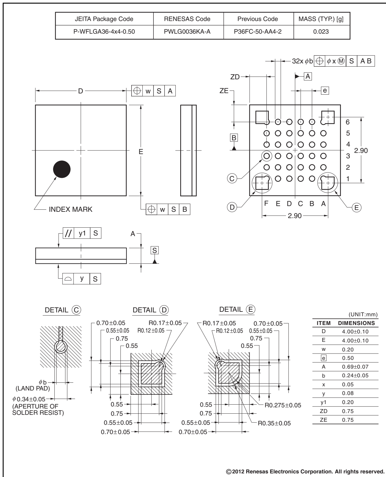
Figure 1.3 LGA 36-pin
