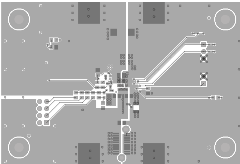
Figure 6 Board layout – layer 4
