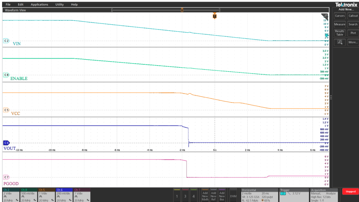
Figure 10 Shutdown with Enable de-assertion at 12A load (Ch2:PV IN , Ch5:V CC , Ch6: V OUT , Ch7: PGood, Ch8: Enable)
