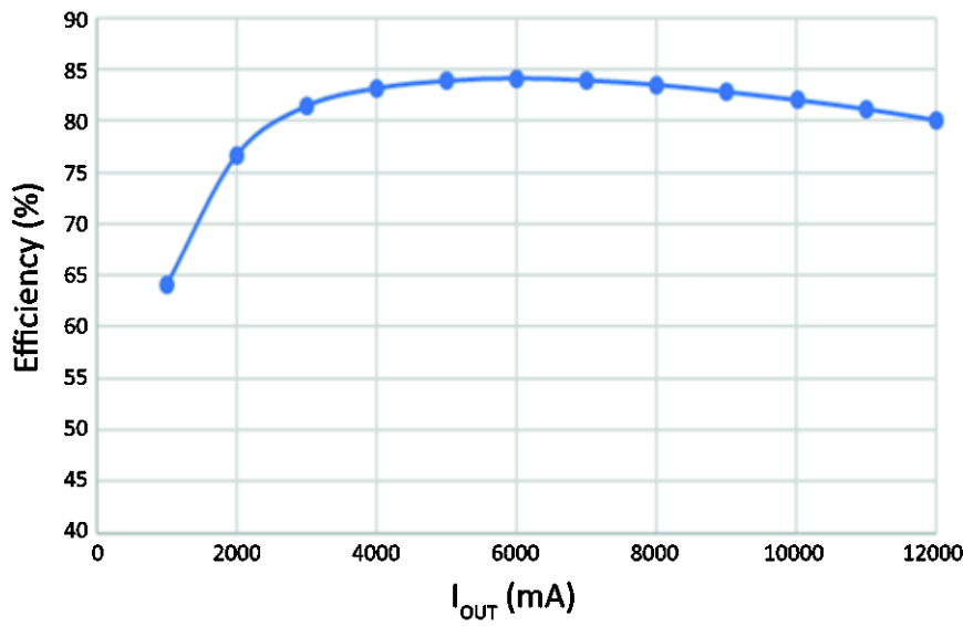
Figure 16 Efficiency
