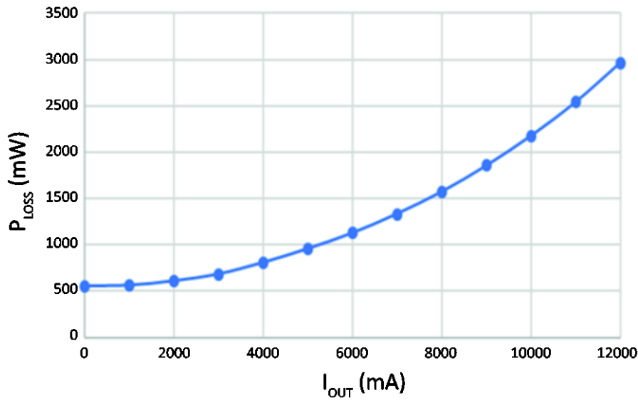
Figure 17 Power loss
