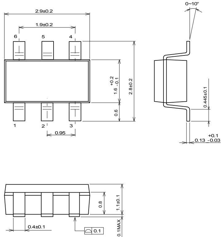
SOT-23-6-1 Package
