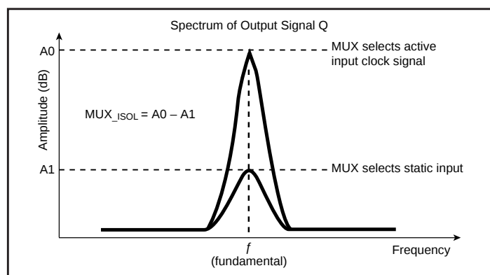
MUX Isolation
