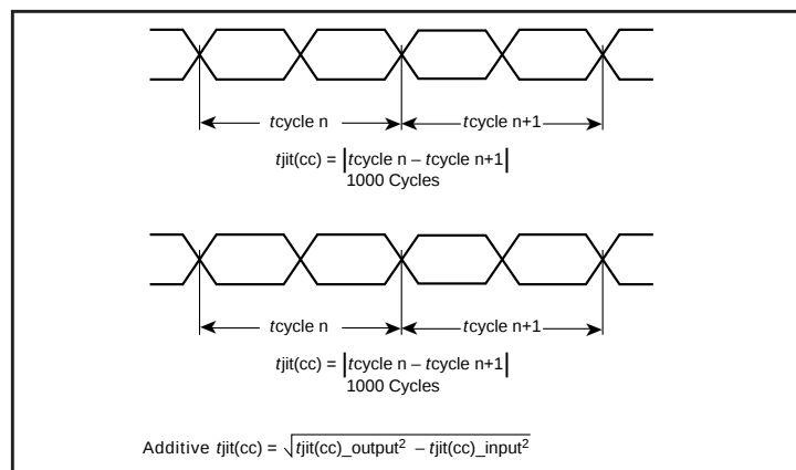
Additive Phase Jitter
