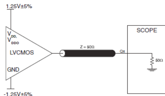
2.5V OUTPUT LOAD AC TEST CIRCUIT
