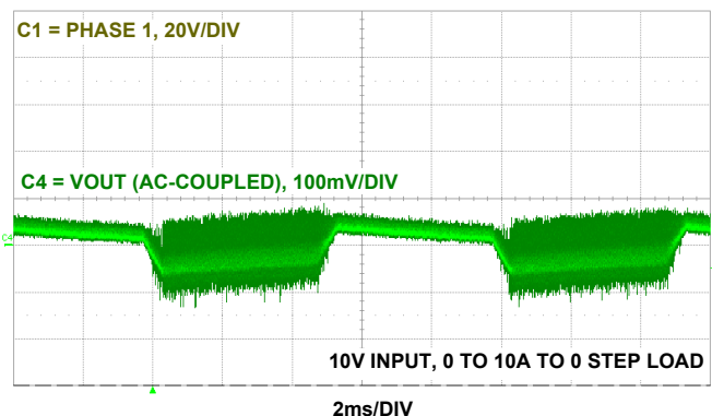
FIGURE 7. FULL STEP LOAD TRANSIENT
