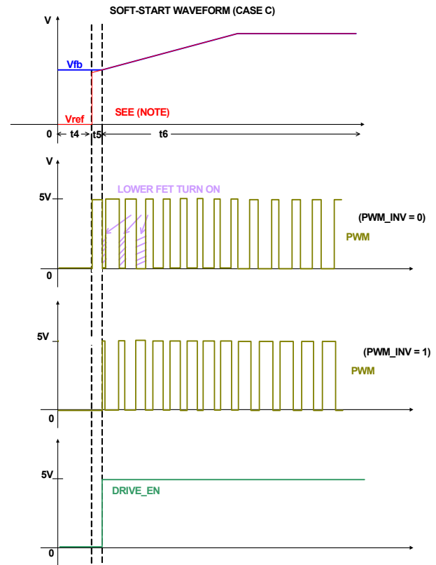
FIGURE 17. SOFT-START WAVEFORM (CASE C, LIGHT LOAD)
