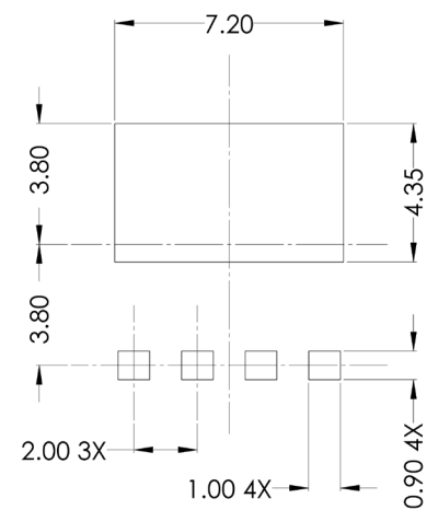
QFN 8X8 Land Pattern
