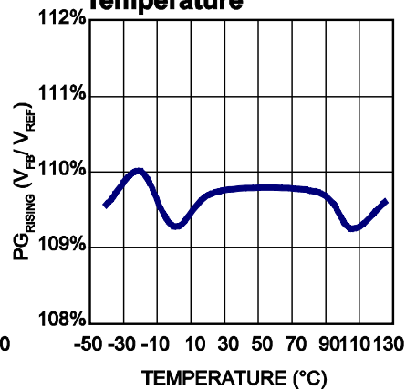
PG Rising Threshold ( V_{FB} Falling) vs. Temperature
