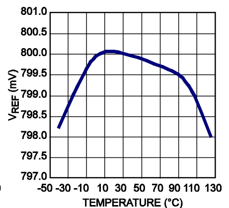
Feedback Reference vs. Temperature
