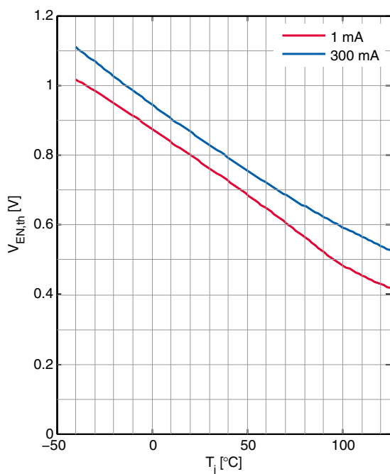
EN Pin Threshold (Off-to-On) versus Junction temperature T_{\text{J}}
