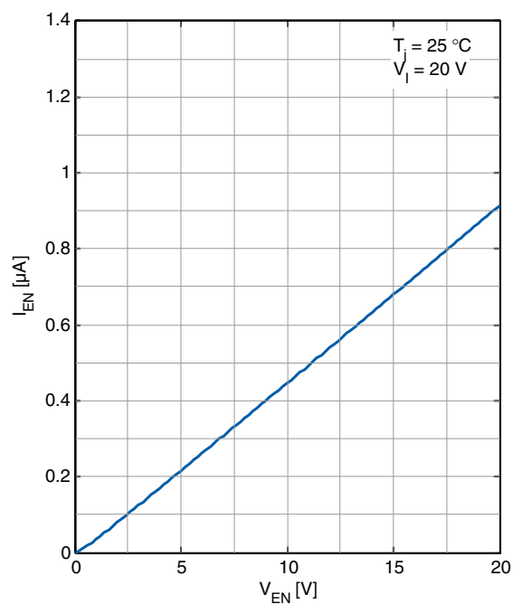
EN Pin Input Current (On-to-Off) versus EN Pin Voltage V_{\text{EN}}
