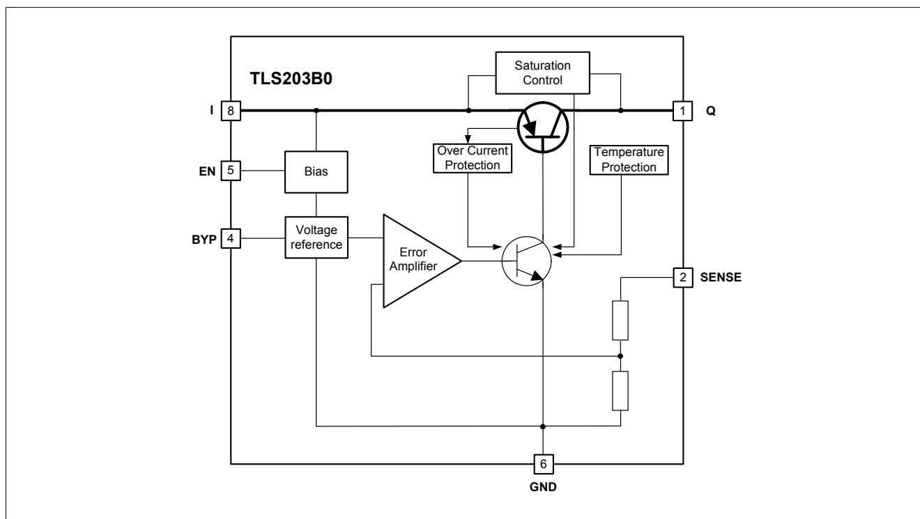
Figure 1 Block Diagram TLS203B0 V33 fixed voltage version
