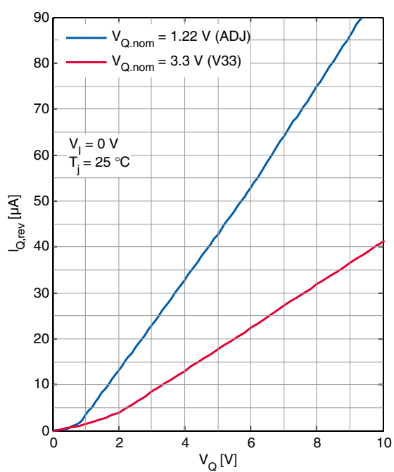
Reverse Output Current versus Output Voltage V_Q
