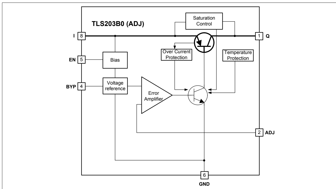
Figure 2 Block Diagram TLS203B0 V adjustable version
