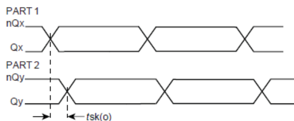
PART-TO-PART SKEW
