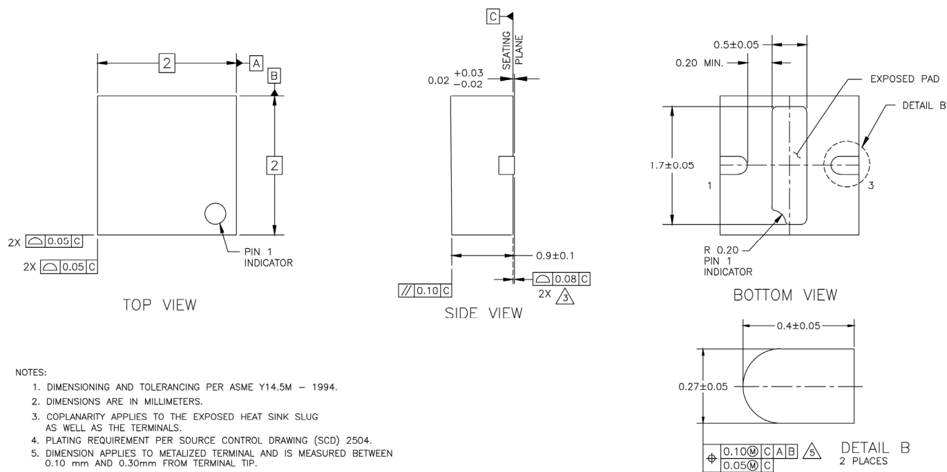
Figure 10. CLA4611-085LF Package Dimensions
