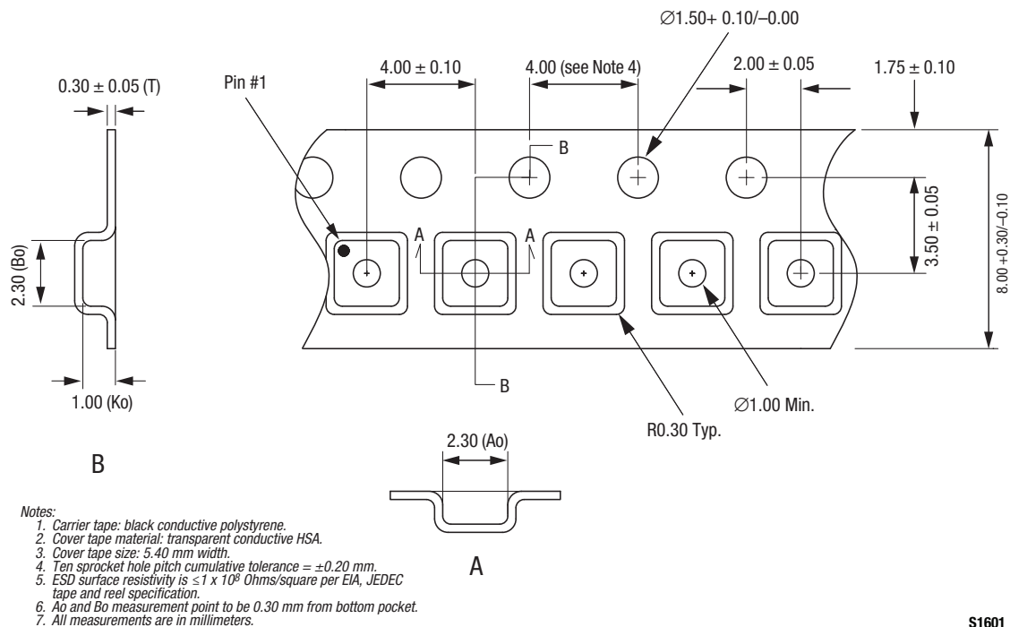
Figure 11. CLA4611-085LF Tape and Reel Dimensions
