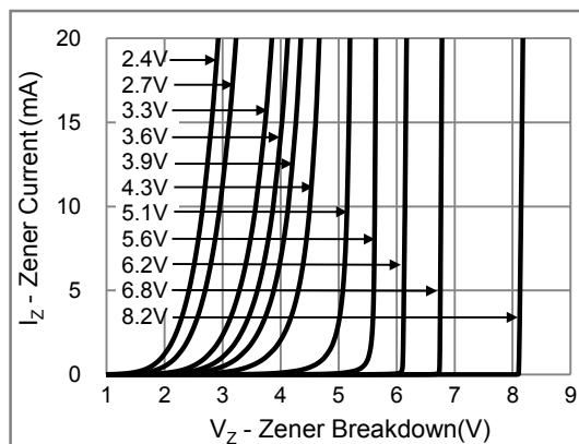
Fig.3 Typical Zener Breakdown
