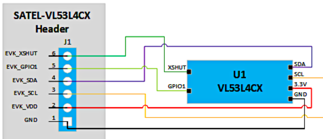
Figure 4. SATEL-VL53L4CX simplified schematic
