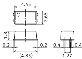
External dimensions
