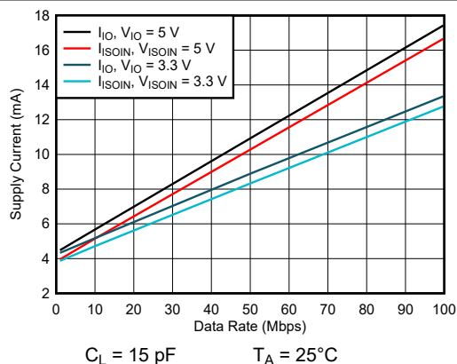
Figure 7-15. ISOW7742 Channel Supply Currents vs Data Rate For C_L = 15 \text{ pF}
