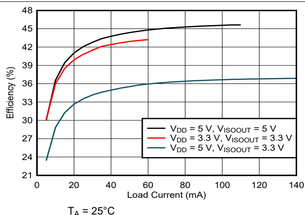
Figure 7-6. Efficiency vs Load Current ( I_{ISOOUT} )
