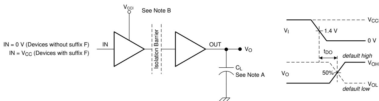
Figure 8-2. Enable/Disable Propagation Delay Time Test Circuit and Waveform
