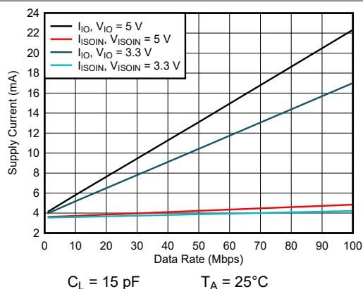
Figure 7-19. ISOW7744 Channel Supply Currents vs Data Rate For C_L = 15 \text{ pF}
