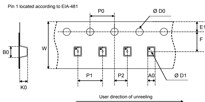
Figure 27. Tape and reel outline
