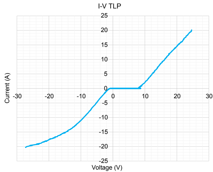
Figure 22. TLP characteristic
