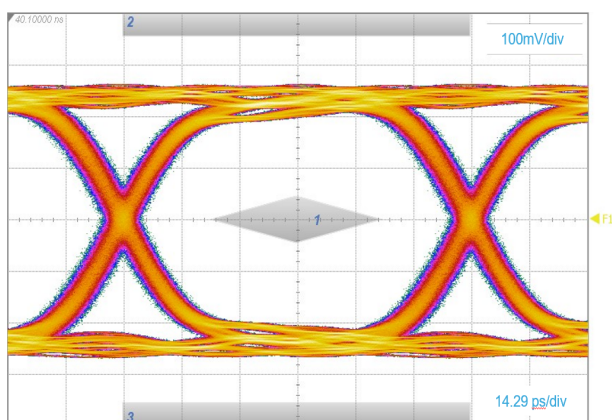
Figure 18. MIPI M-PHY – Gear 4 at 11.66 Gbps eye diagram without ECMFx-40A100Nx
