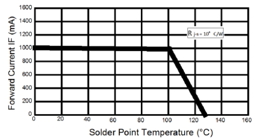
Thermal Design for De-rating
