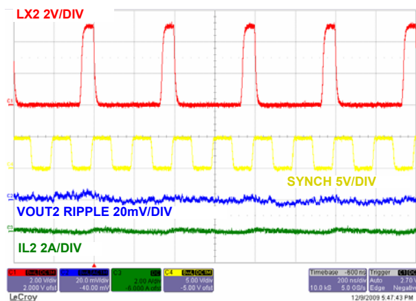
FIGURE 26. STEADY STATE OPERATION CHANNEL 2 AT NO LOAD WITH F_{SW} = 5MHz
