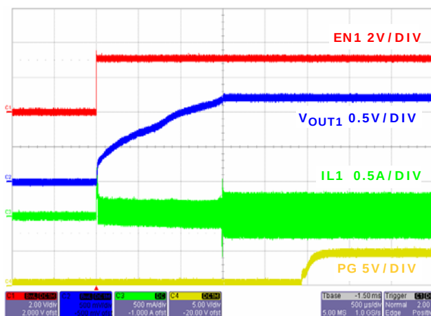
FIGURE 18. SOFT-START WITH NO LOAD CHANNEL 1
