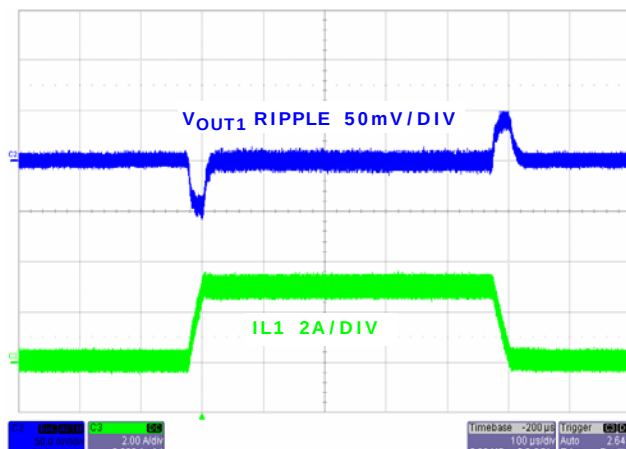
FIGURE 16. LOAD TRANSIENT CHANNEL 1 (PWM)
