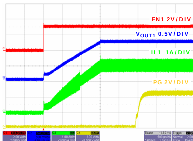
FIGURE 20. SOFT-START AT FULL LOAD CHANNEL 1
