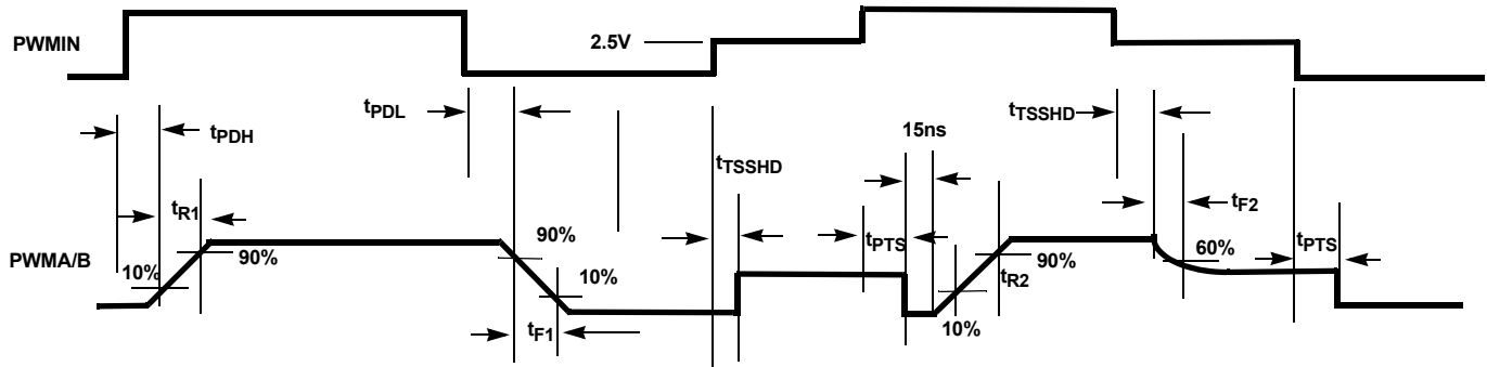
FIGURE 1. TIMING DIAGRAM
