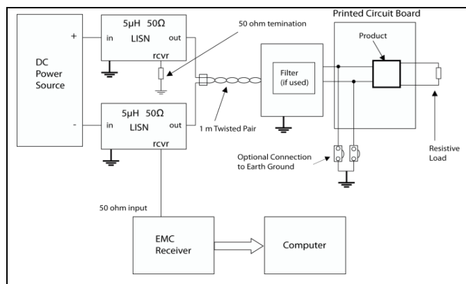
Test set-up
