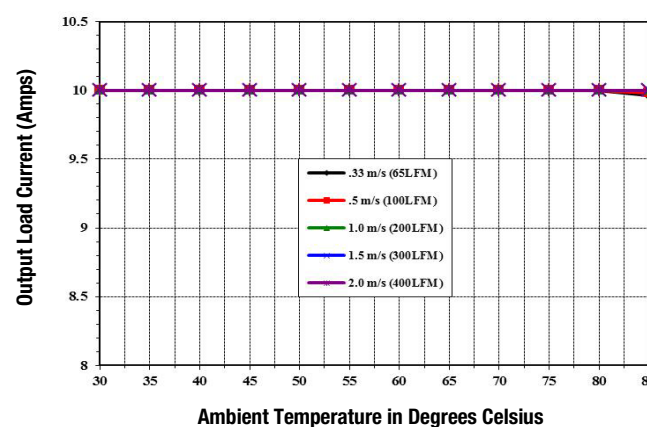
UWS-5/10-Q12N-C Temperature Derating Vin 30V (Airflow from Pin 1 to Pin 3 on PCB)
