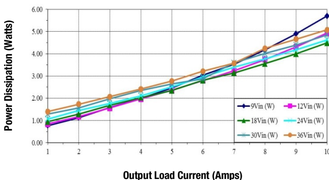
UWS-5/10-Q12N-C Power Dissipation vs. Line and Load
