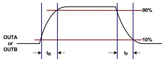
Figure 5. Rise/Fall Times
