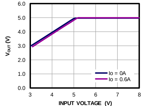
Dropout Performance
