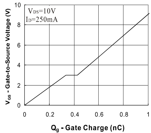
Fig.7 - Gate Charge
