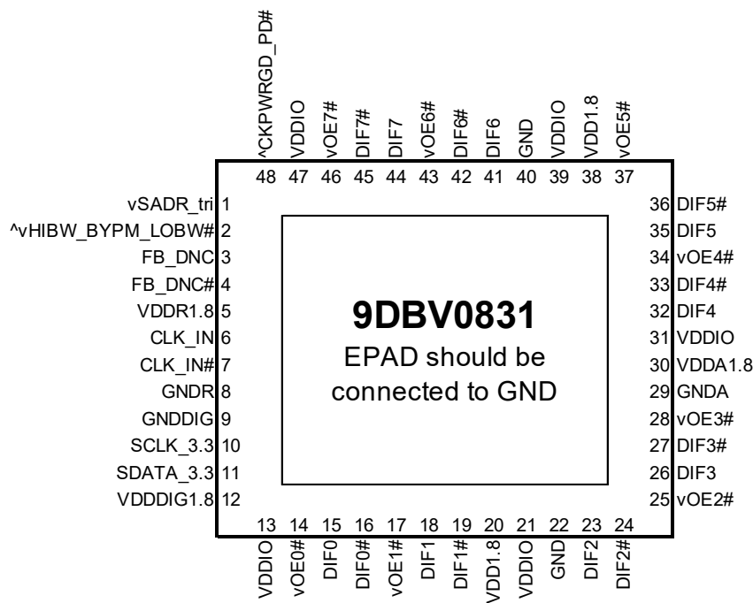
48-pin VFQFPN, 6x6 mm, 0.4mm pitch
