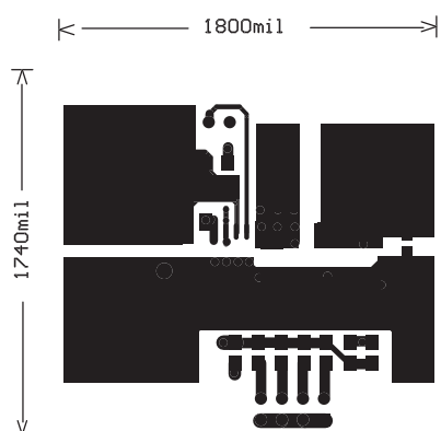
Figure 6c. Top-Side Copper
