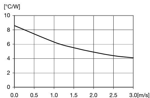
Thermal resistance vs. airspeed measured at the converter. Tested in wind tunnel with airflow and test conditions as per the Thermal consideration section. V_i = 53\text{ V} .
