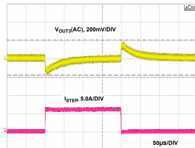
FIGURE 25. PWM3 LOAD TRANSIENT RESPONSE (LOAD STEP FROM 3A TO 9A)
