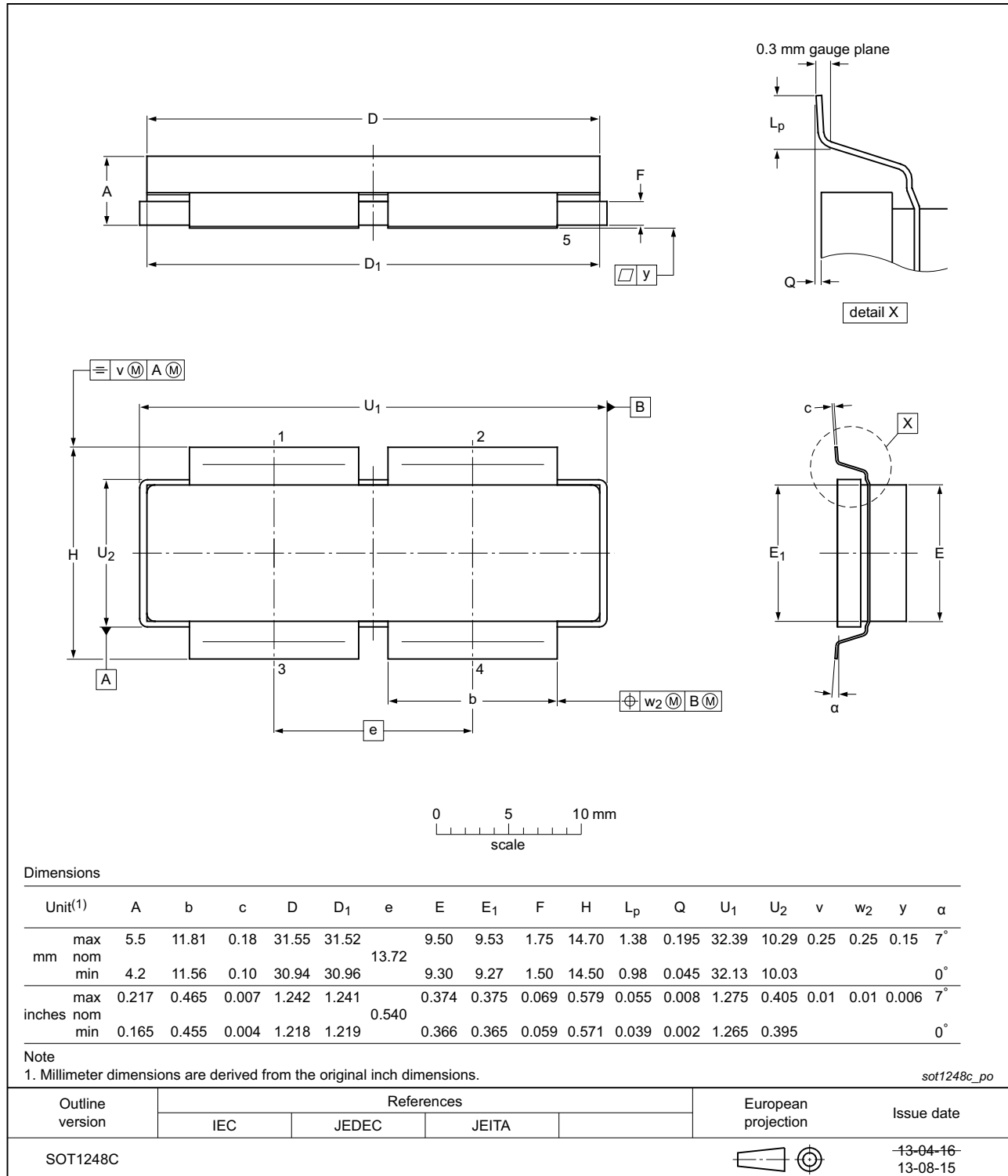
Fig 13. Package outline SOT1248C
