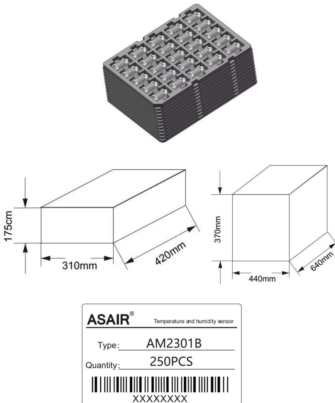
Figure 14. Schematic diagram of packaging
