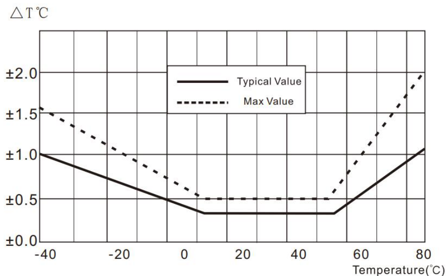
Figure 3. Typical and maximum temperature errors
