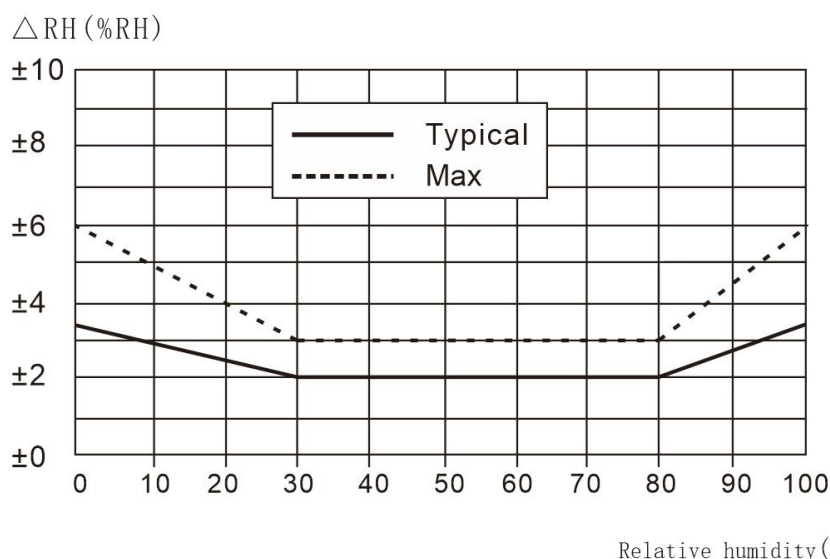
Figure 2. Typical and maximum humidity errors
