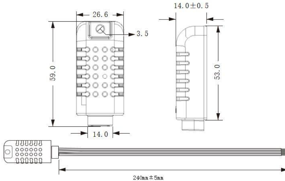
Figure 12. AM2301B sensor encapsulation (unit: mm not specified tolerance: \pm 0.2 mm)
