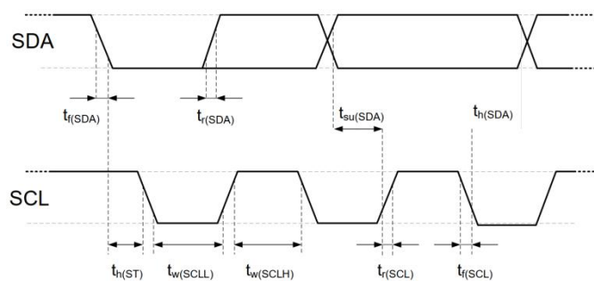
Figure 9. Timing diagram of digital input / output
