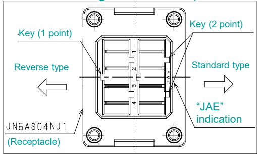
Connector Pulling Out Direction (for reference)
