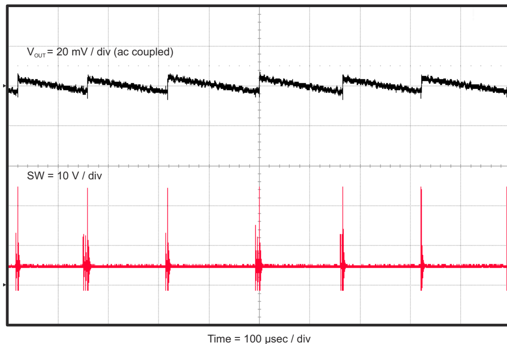
Figure 2-9. TPS54335AEVM-010 Output Ripple, I_{OUT} = 0 A
