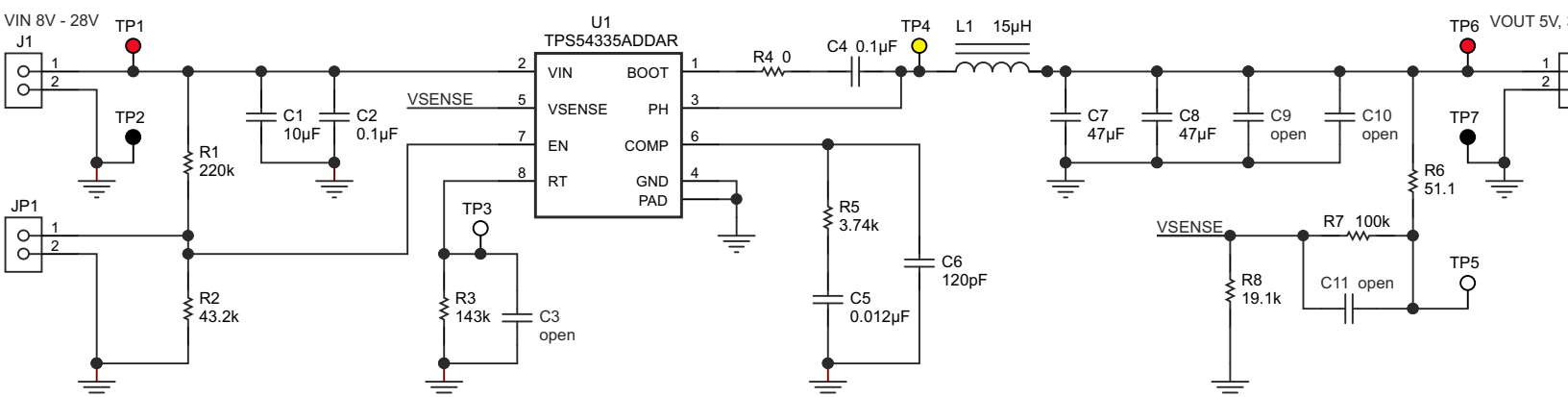
Figure 4-1. TPS54335AEVM-010 Schematic
