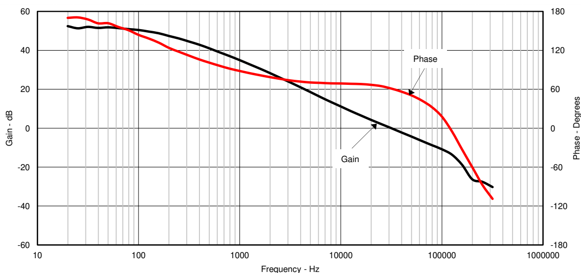
Figure 2-6. TPS54335AEVM-010 Loop Response
