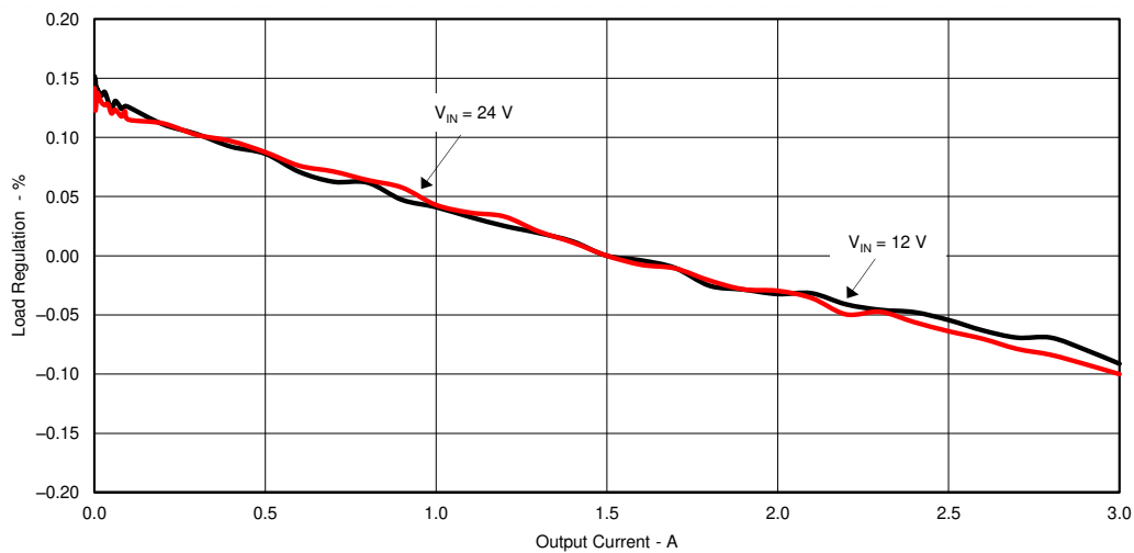
Figure 2-3. TPS54335AEVM-010 Load Regulation
