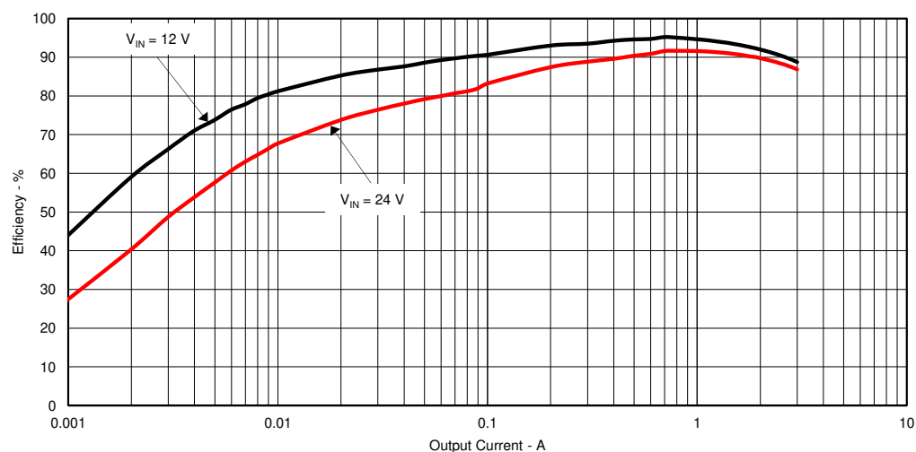
Figure 2-2. TPS54335AEVM-010 Low Current Efficiency
