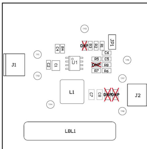
Figure 3-1. TPS54335AEVM-010 Top-Side Assembly
