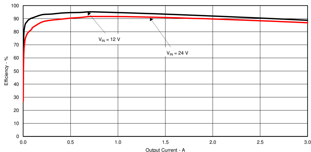
Figure 2-1. TPS54335AEVM-010 Efficiency
