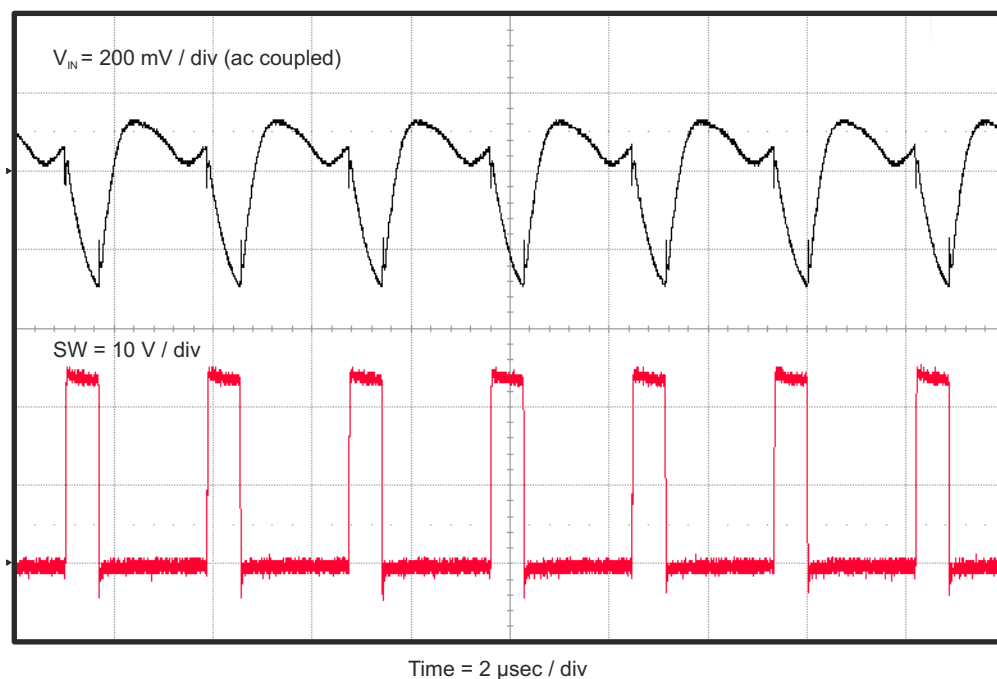
Figure 2-10. TPS54335AEVM-010 Input Ripple
