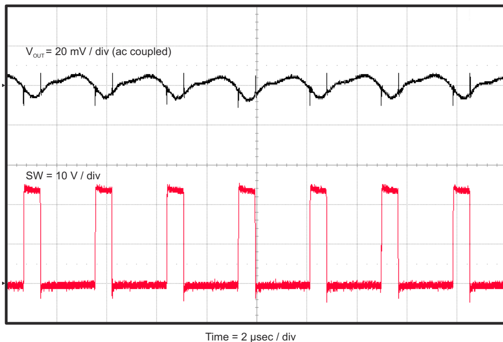
Figure 2-7. TPS54335AEVM-010 Output Ripple, I_{OUT} = 3 A
