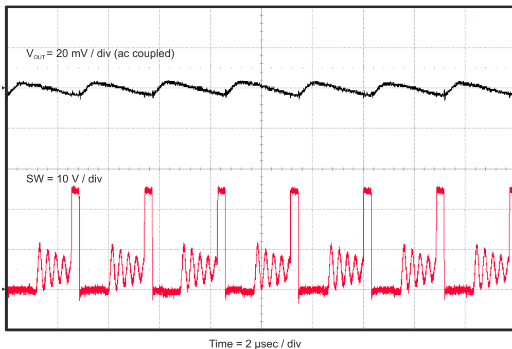
Figure 2-8. TPS54335AEVM-010 Output Ripple, I_{OUT} = 100 mA
