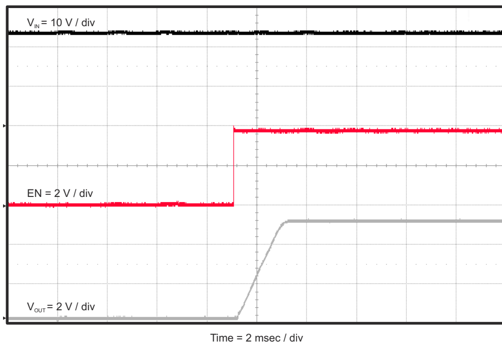
Figure 2-12. TPS54335AEVM-010 Start-up Relative to Enable
