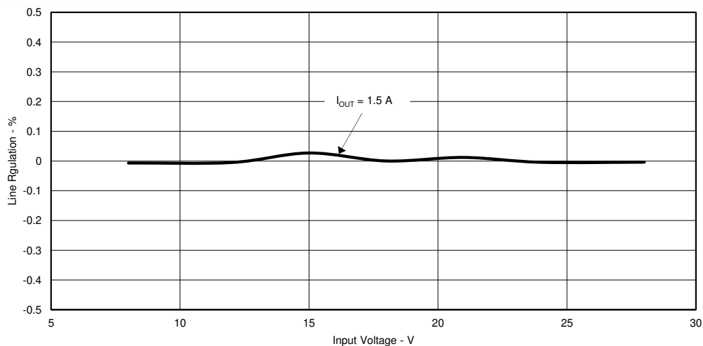
Figure 2-4. TPS54335AEVM-010 Line Regulation
