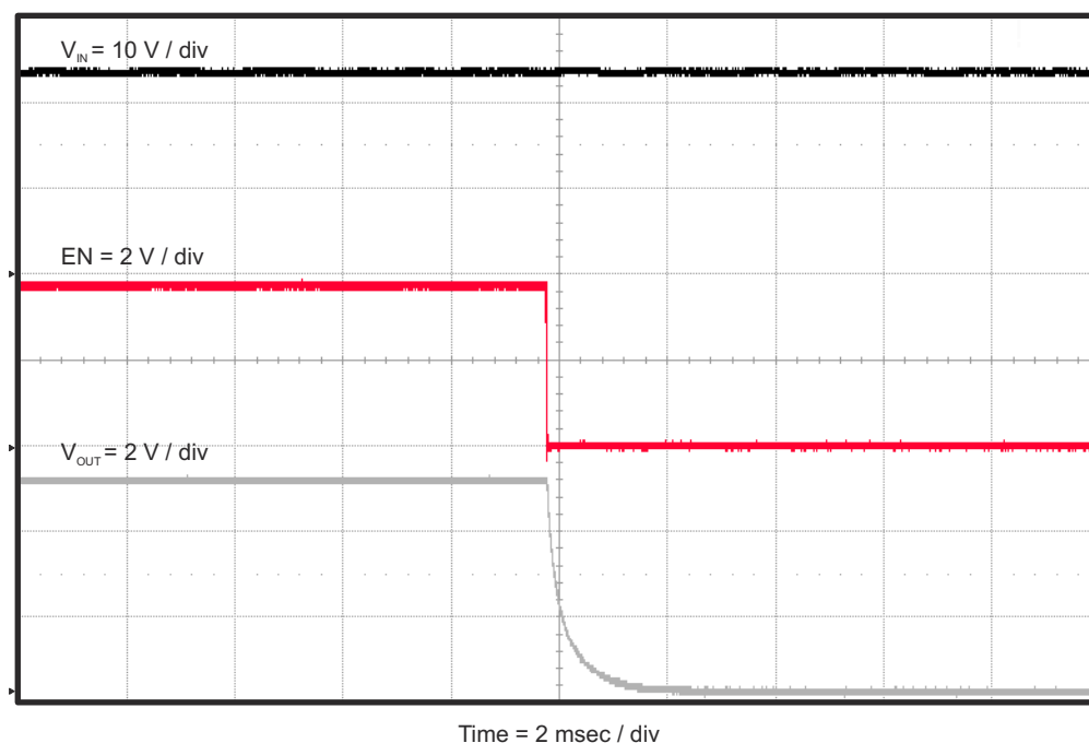
Figure 2-14. TPS54335AEVM-010 Shut-down Relative to EN
