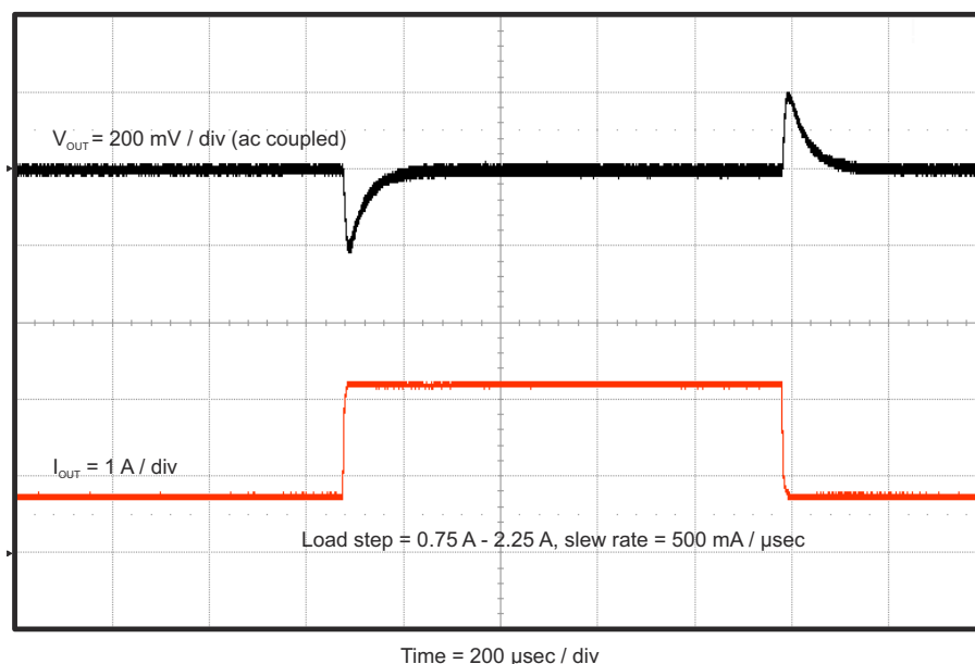
Figure 2-5. TPS54335AEVM-010 Transient Response
