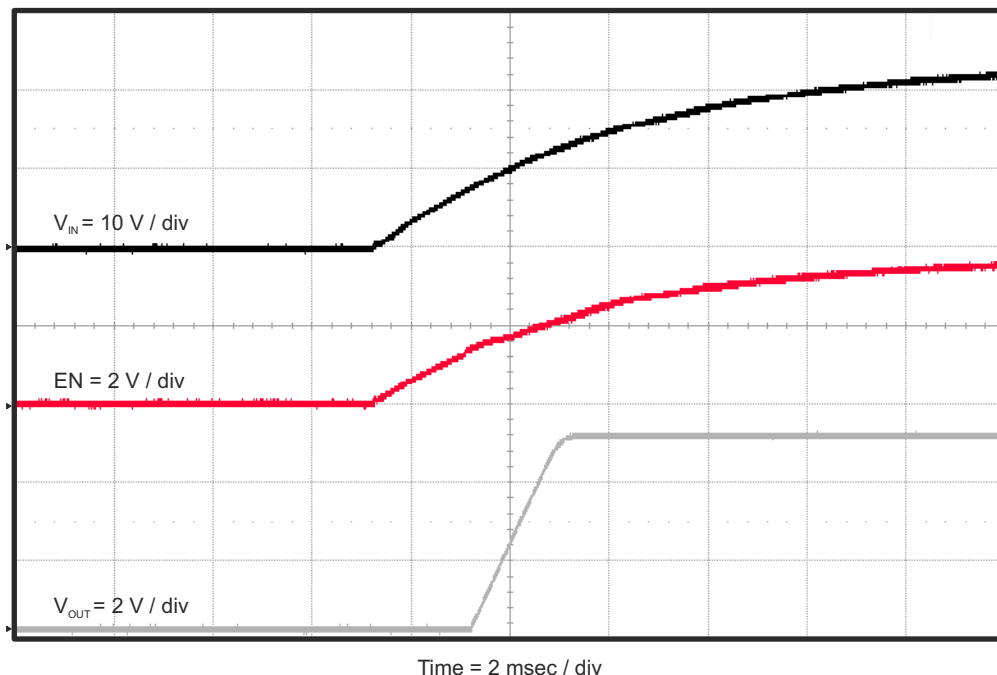
Figure 2-11. TPS54335AEVM-010 Start-Up Relative to V_{IN}
