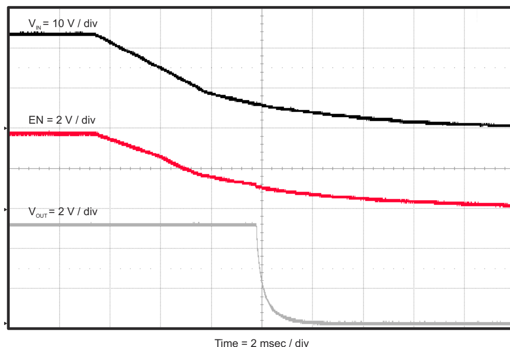
Figure 2-13. TPS54335AEVM-010 Shut-down Relative to V_{IN}
