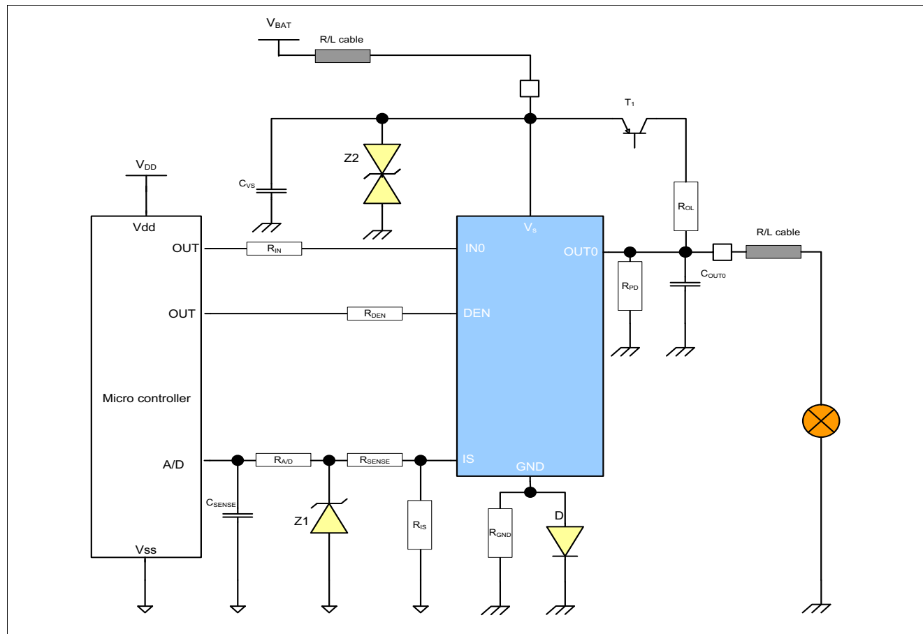
Figure 52 Application Diagram with BTS5090-1EJA
