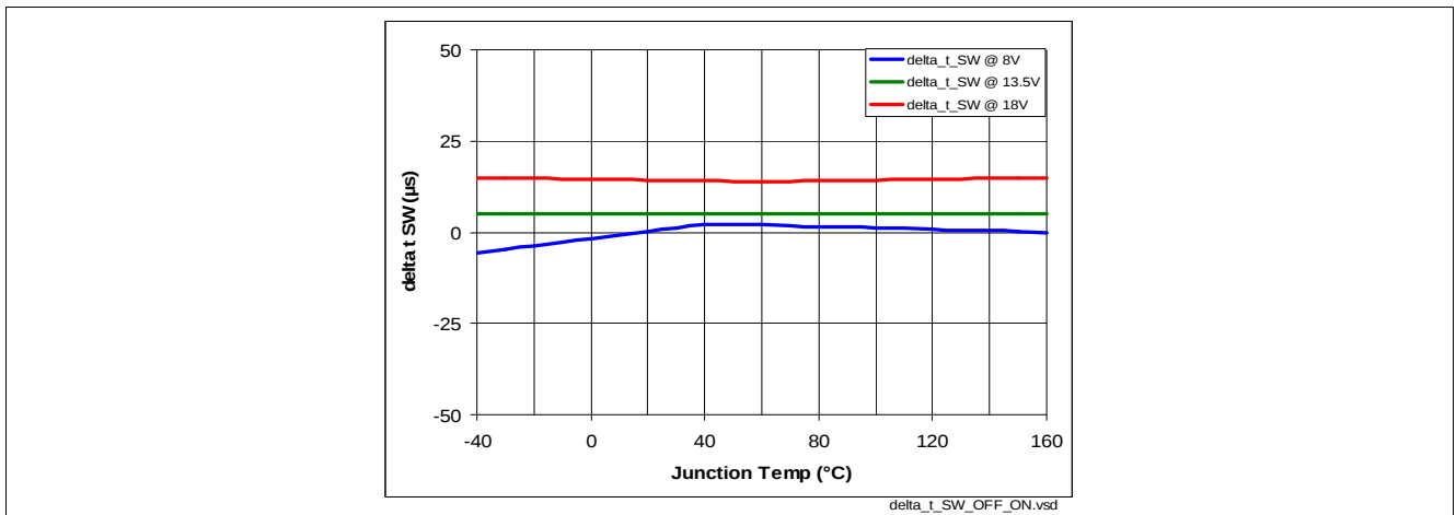
Figure 39 Turn ON / OFF matching \Delta t_{\text{SW}} = f(T_J; V_S) , R_L = 6 \Omega
