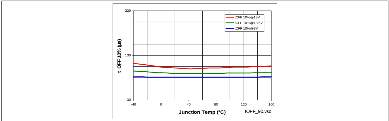
Figure 38 Turn OFF t_{\text{OFF}} = f(T_J; V_S) , R_L = 6 \Omega
