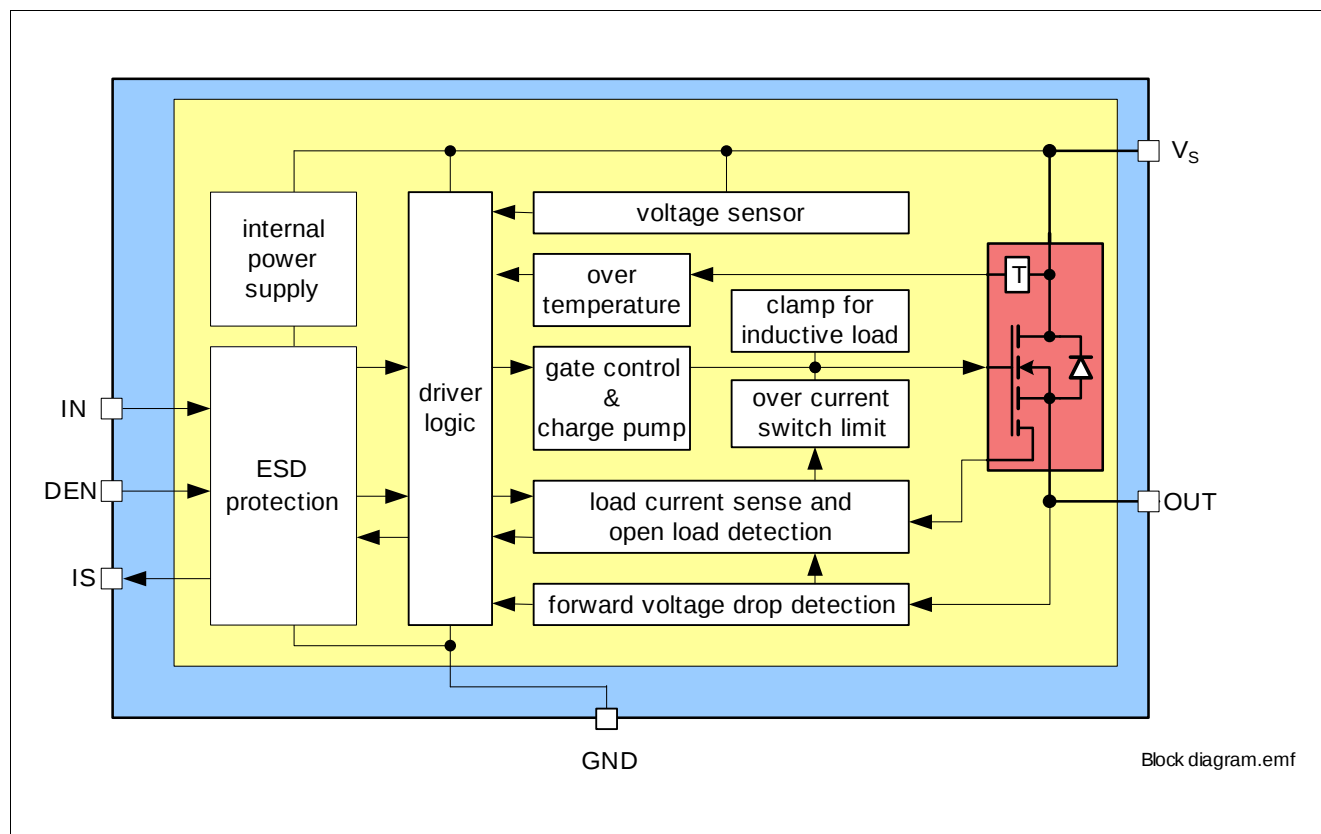
Figure 1 Block Diagram for the BTS5090-1EJA
