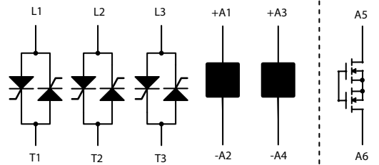
DR6760X60 (3 CONTROLLED LEGS)
