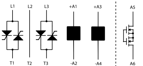
DR6760X75 (2 CONTROLLED LEGS)
