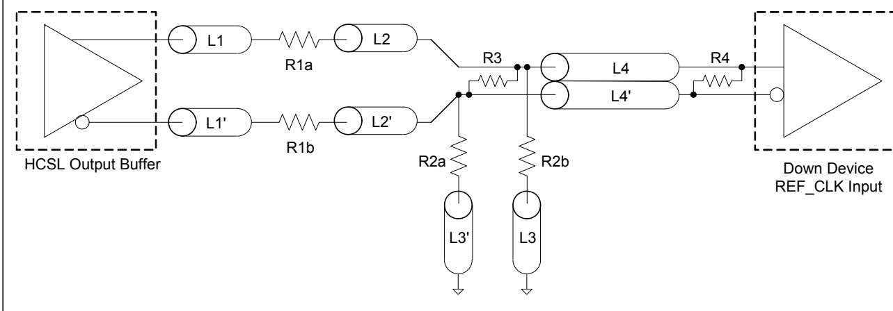
Termination for Cable AC Coupled Application (figure 4)
