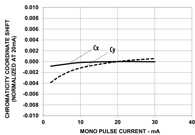
Figure 6: Chromaticity Coordinate Shift vs. Mono Pulse Current (2700K)
