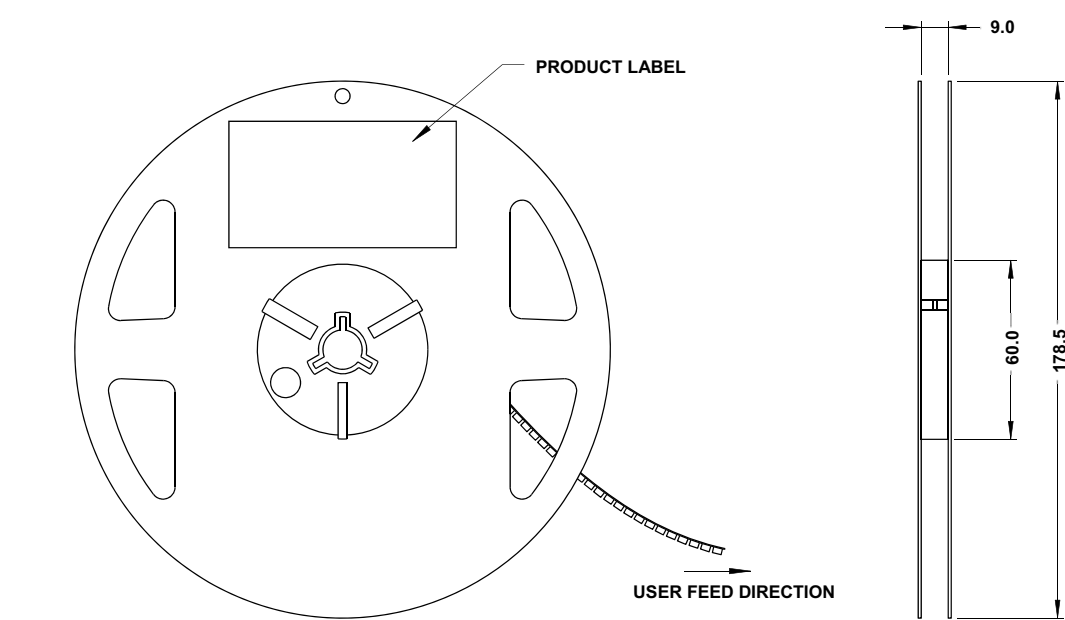
Figure 18: Reel Dimensions
