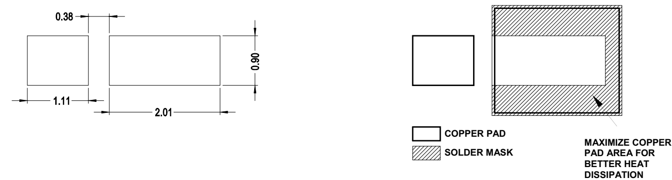
Figure 16: Recommended Soldering Land Pattern
