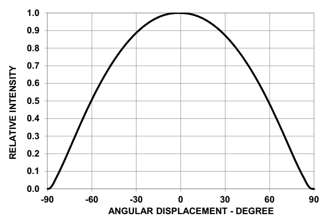
Figure 5: Radiation Pattern
