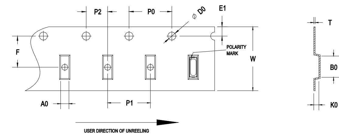
Figure 17: Carrier Tape Dimensions
