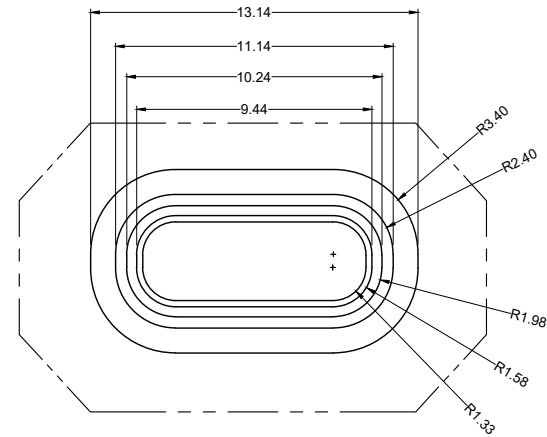
Recommended Panel Opening Dimensions Tolerance \pm 0.03\text{mm}
