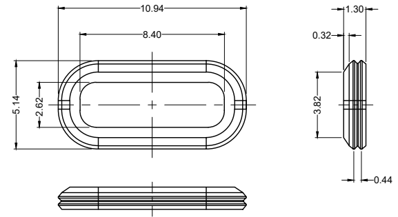
Gasket Detail Material: Silicone, Black
