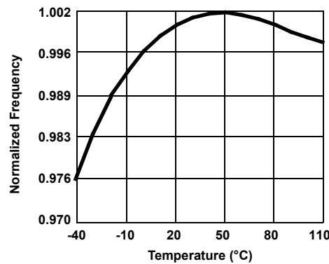
Figure 5. Oscillator Frequency vs Temperature
