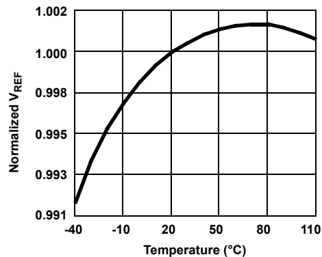
Figure 4. VREF Reference Voltage vs Temperature
