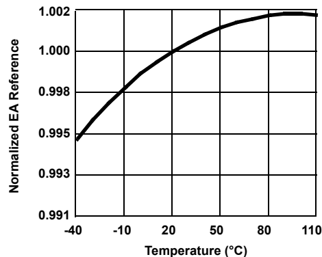
Figure 3. EA Reference Voltage vs Temperature
