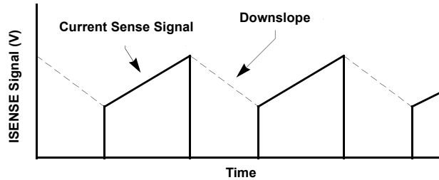
Figure 7. Slope Compensation
